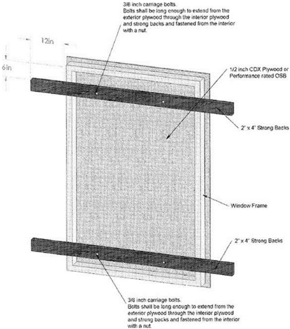
FIGURE A103.1(1) BOARDING OF DOOR OR WINDOW
